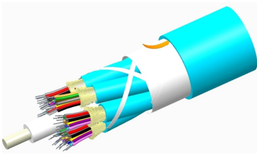
LazrSPEED® Low Smoke Zero Halogen Riser Distribution Cable, 48 fiber multi-unit with 12 fiber subunits
